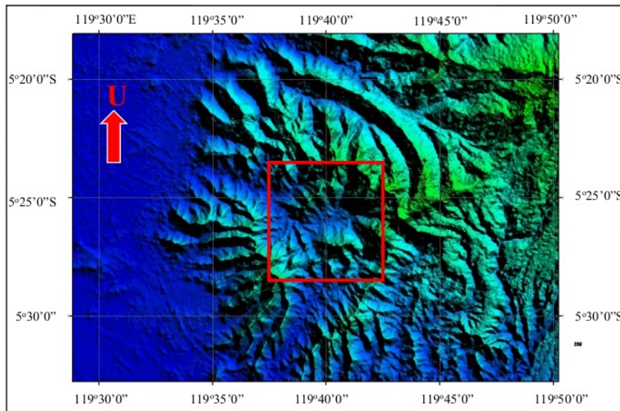
FIGURE 4. The crater structure of Sapaya volcano (square)
