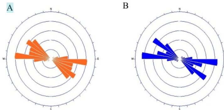
4 FIGURE 3. (A) Rosette diagram of Lineament of highland areas, (B) Lineament of lowland areas.
